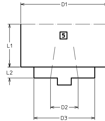
Mandrino ISO ISO Spindle
