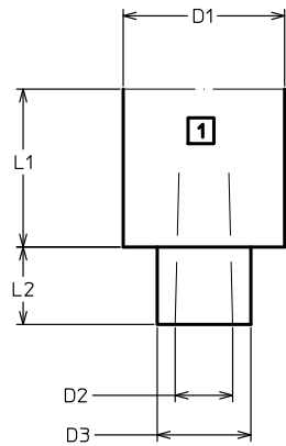
Mandrino CM MT Spindle
