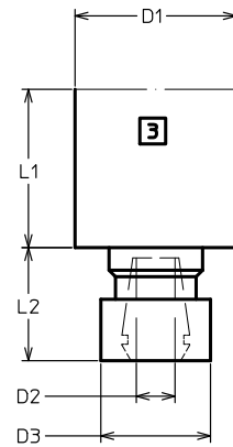
Mandrino a Pinza Collet Spindle
